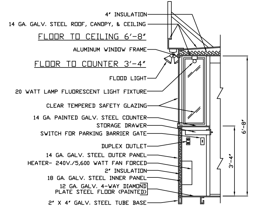
S1 SECTION NO SCALE (BOOTH SECTION ONLY)
