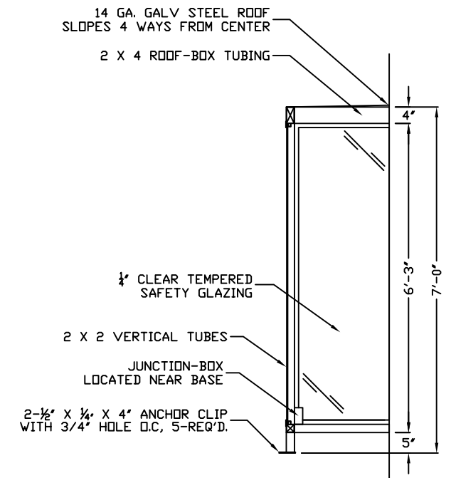
S1 SECTION
