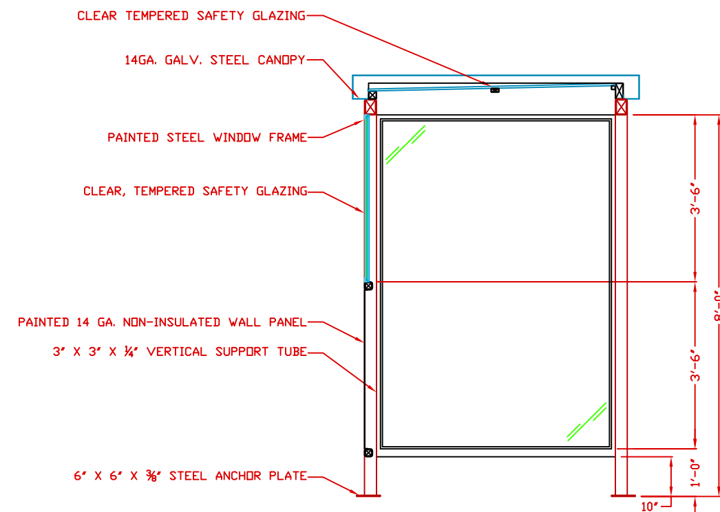
S1 SECTION NO SCALE
