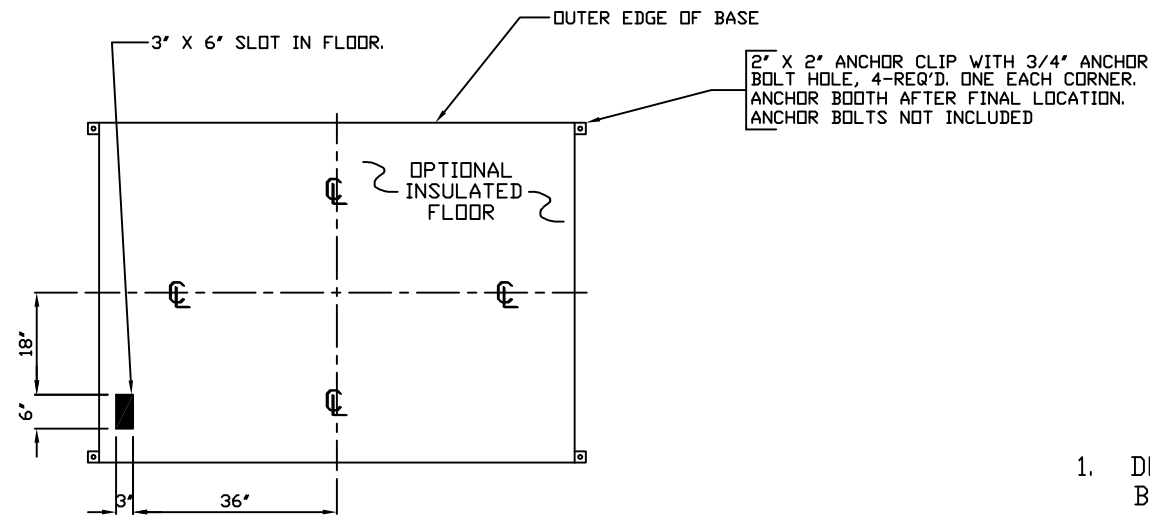
SERVICE ENTRANCE/ANCHOR BOLT LAYOUT
