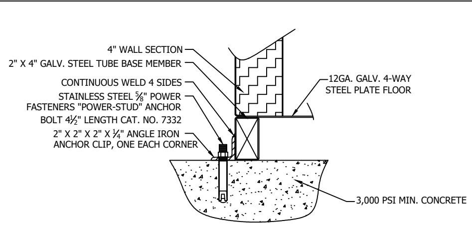
FIELD DRILLED ANCHOR BOLT DETAIL NO SCALE
