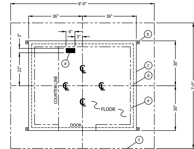
SERVICE ENTRANCE/ANCHOR BOLT LAYOUT
