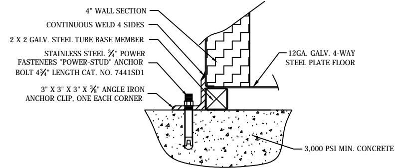
FIELD DRILLED ANCHOR BOLT DETAIL NO SCALE
