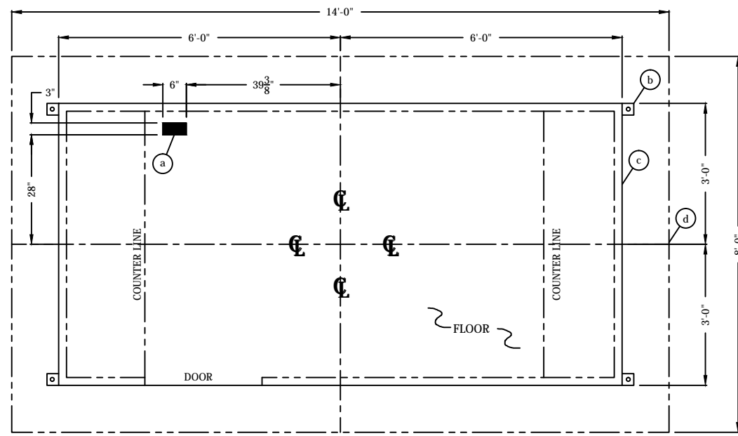
SERVICE ENTRANCE/ANCHOR BOLT LAYOUT
