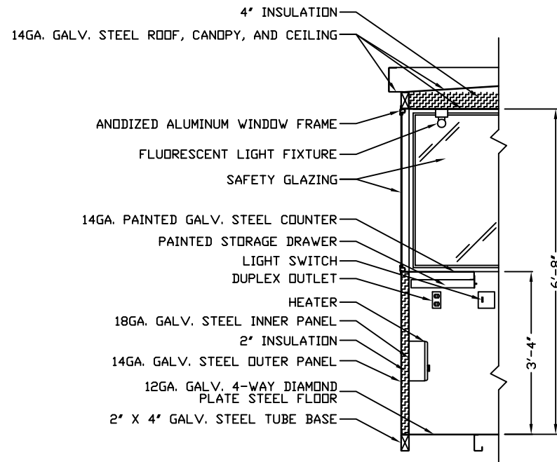
(S1) SECTION NO SCALE
